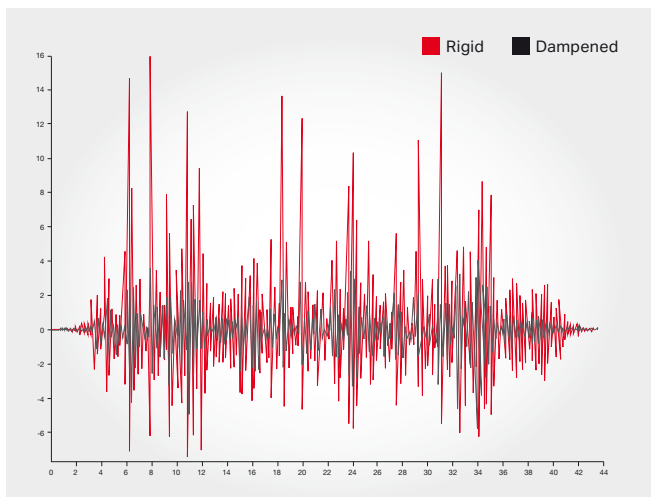
Reductions of vibrations in the vertical direction with/without Komatsu Comfort Ride
